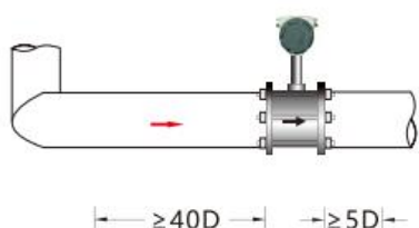
Two 90-degree bends in different planes
