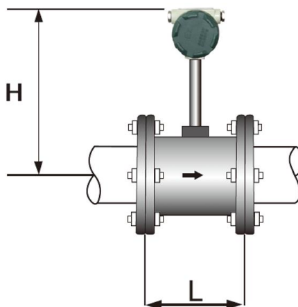
Fig.2 Installation diagram of flange type
