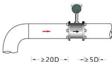
A 90-degree bend
