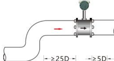
Two 90-degree bends in the same plane
