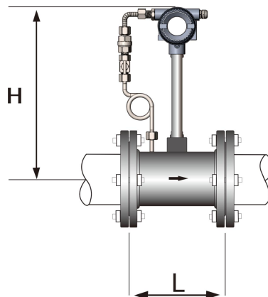
Fig.2 Installation diagram of Temperature & Pressure Compensation type
