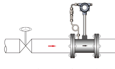
Adjustment valve semi-open valve (not recommended)
