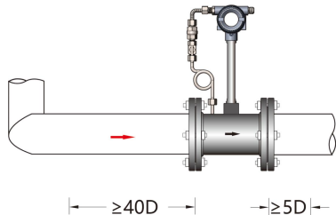
Two 90-degree bends in different planes
