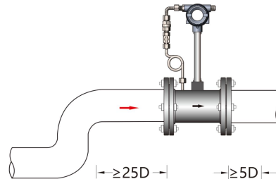
Two 90-degree bends in the same plane
