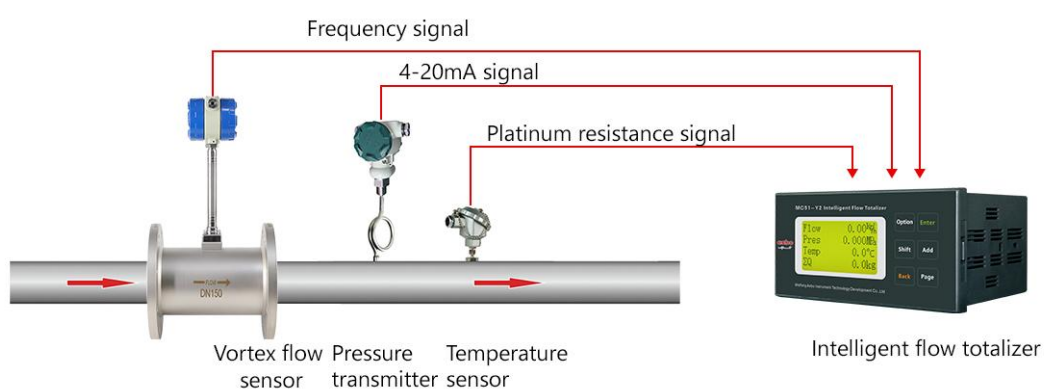
Installation Diagram
