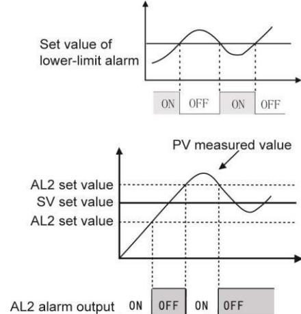
Deviation external alarm output
