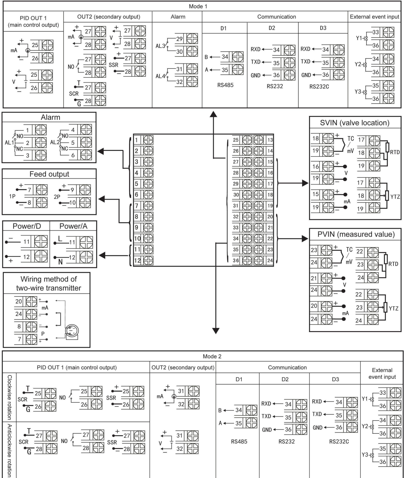
Wiring diagram type A, B, C, D, E, K, L and M
