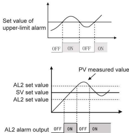
Deviation internal alarm output
