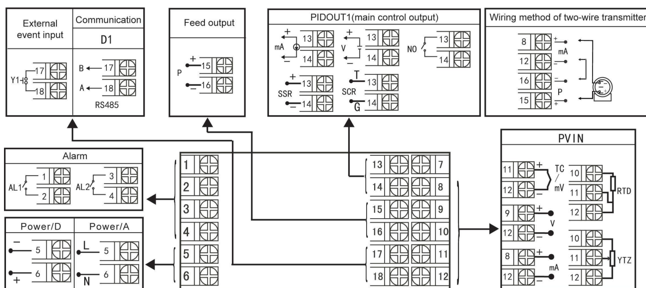
Wiring Diagram of Type H
