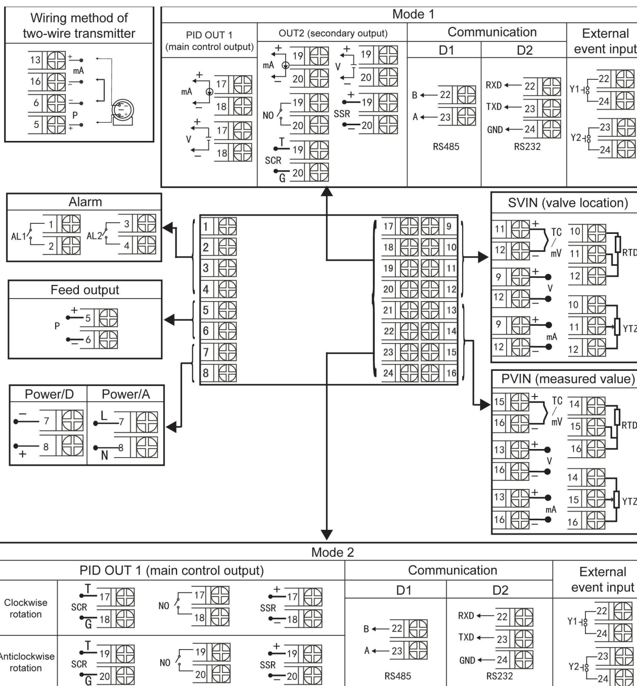
Wiring Diagram of Type F
